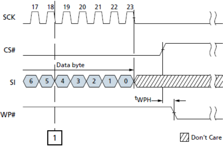
WP# Timing
