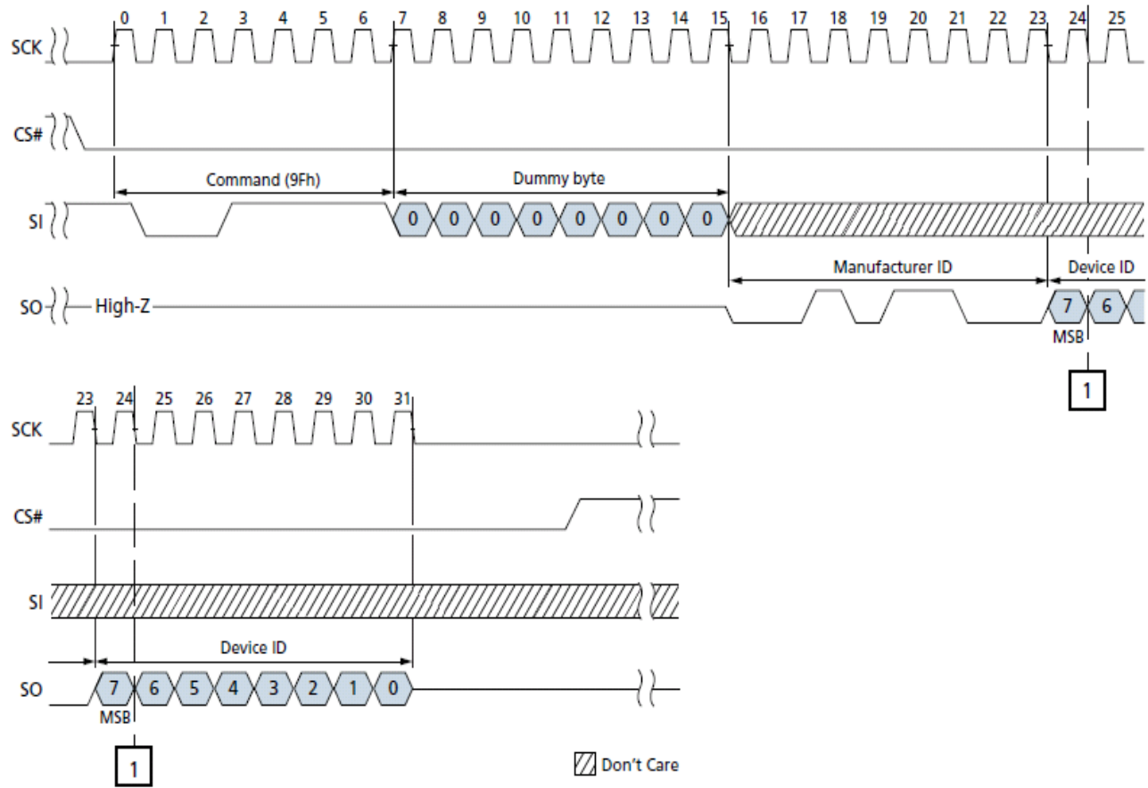
READ ID (9Fh) Timing
