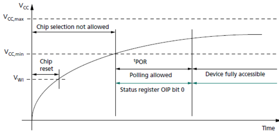
SPI Power-Up
